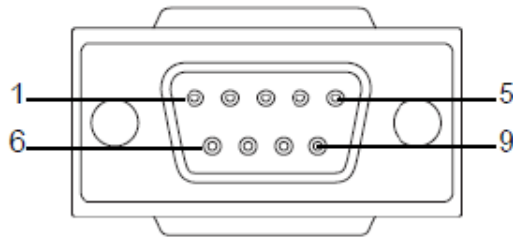
Figure 2.11 DB9 Pin Assignment
